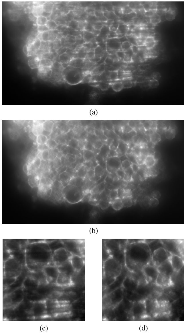
Fig. 11. SPIM images of a Multicellular Tumor Spheroid stained with DiI acquired with an objective 20X NA 0.5, an excitation wavelength of 532 nm and an emission wavelength of 593 nm. The voxel size is 0.32 \times 0.32 \times 1 \mu\text{m} . (a) Single plane of a 3D stack; (c) A magnified view of a region of (a); (b) Denoised image; (d) A magnified view of the same region of (b).
