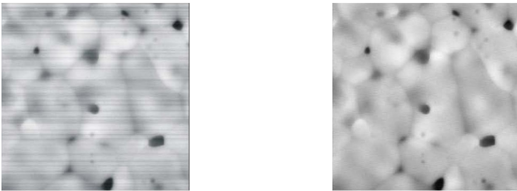
Fig. 10. SEM imaging on a sintered specimen of \text{CeO}_2 (cerium oxide) at a sintering temperature of 1400 C for 2 hours and 50 minutes [8]. The image is composed of 512x512 pixels with each side measuring 70.55 \mu\text{m} ; the intensity unit is 0.1 \mu\text{m} .
